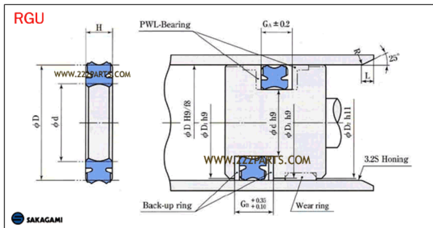
Dimension table of RGU-Packings
