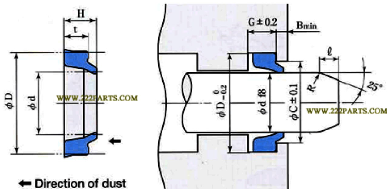
Dimension table of SFR-Wipers
